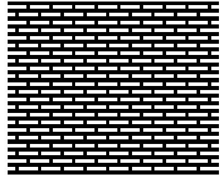
Nr. 4183 mm hole width b x h 5,0 x 0,8 pitch horizontal 5,9 pitch vertical 2,0+2,0 opening 34 %
