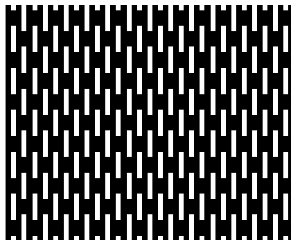
Nr. 4305 mm hole width b x h 0,85 x 5,0 pitch horizontal 2,0+2,0 pitch vertical 8,0 opening 26,5 %
