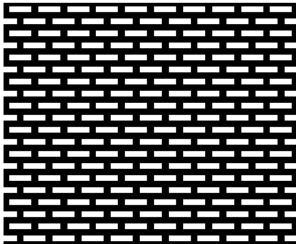
Nr. 1490 mm hole width b x h 4,0 x 1,0 pitch horizontal 5,4 pitch vertical 2,25+2,25 opening 33 %
